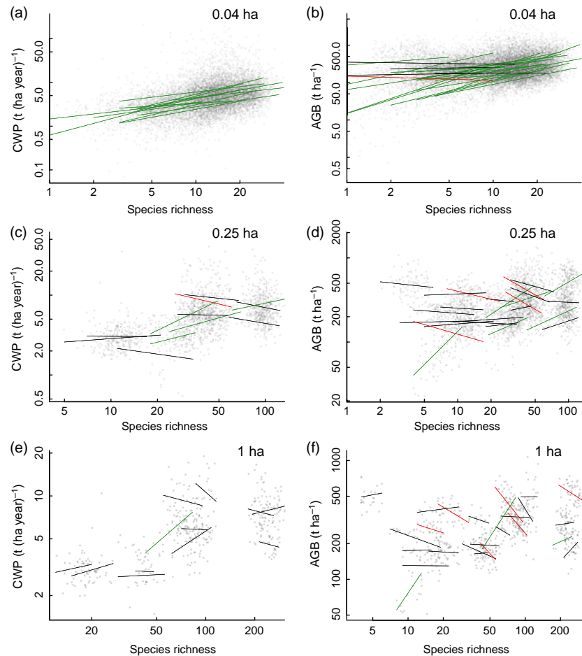
Fig. 2. Observed relationships of tree species richness to coarse woody productivity (CWP; panels a, c, e) and above-ground biomass (AGB; panels b, d, f) at the study sites at three spatial grains (0.04 ha, 0.25 ha, 1 ha). Points show the quadrat data (number of points for each site = site area/spatial grain; see Table 1), lines show regressions for individual sites, with green indicating positive slopes, red negative slopes and black slopes not significantly different from zero. Axis scales are logarithmic.
